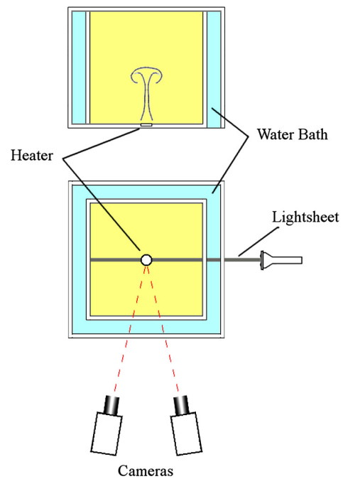
Fig. 1. Elevation (top) and plan view (bottom) of the test-section and PIV system.
