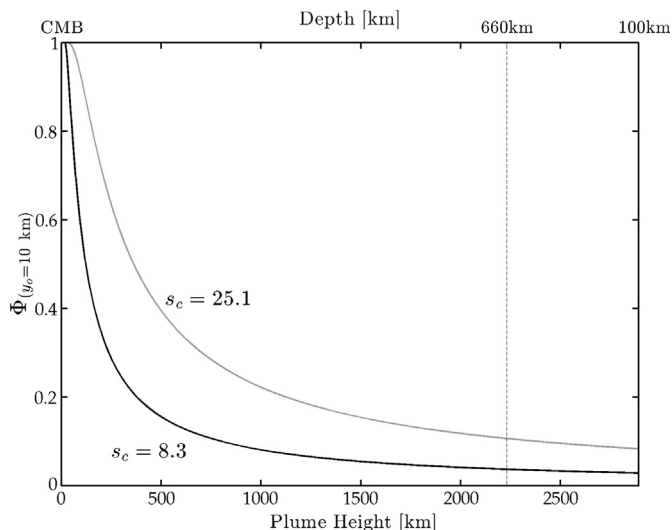
Fig. 9. Proportion of a plume derived from the lowermost 10 km in the mantle as a function of plume height for two different values of the sampling coefficient.
