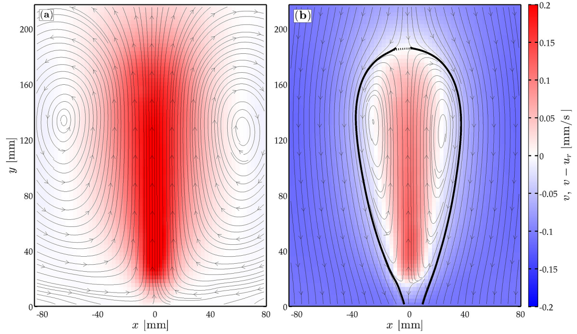
Fig. 2. Contours of the vertical velocity and streamlines at t = 1797 s and Ra = 1.36 \times 10^6 , computed in an Eulerian reference frame (a) and one moving with the plume (b). The thick black line in (b) represents the vortex ring bubble.
