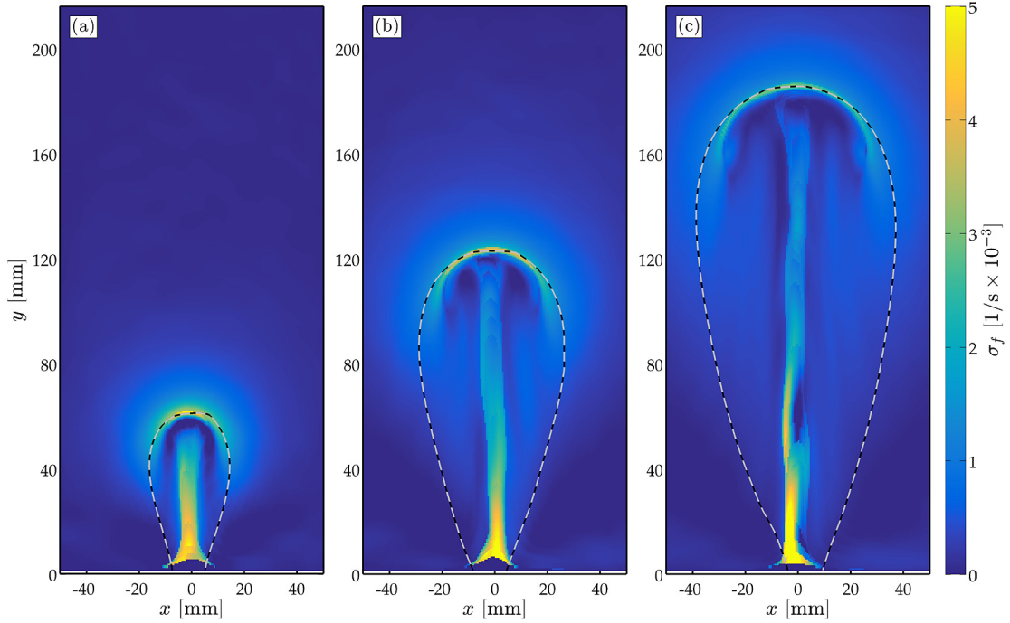
Fig. 4. Finite-Time Lyapunov Exponent fields computed at y_p = 60.8 mm (a), 122.1 mm (b), and 185.2 mm (c), for Ra = 1.36 \times 10^6 . The vortex ring bubble is shown by the black and white dashed lines, and aligns with ridge at the top of the plume head.
