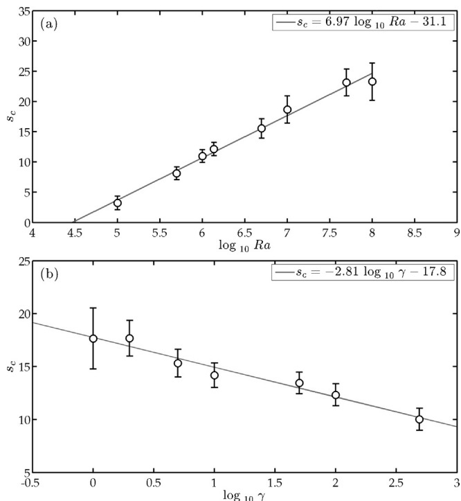
Fig. 8. Variation in the predicted sampling coefficient of plumes as a function of Rayleigh number at \gamma = 141.4 (a), and as a function of viscosity contrast at Ra = 1.36 \times 10^6 (b). The grey lines represent the best-fit linear trend between s_c and the log values.
