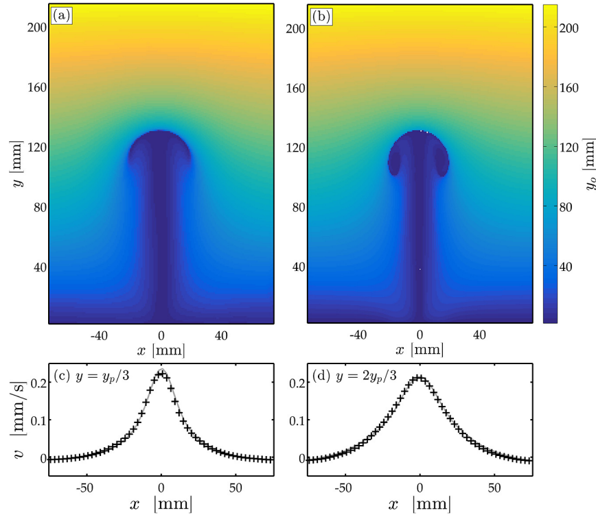
Fig. 7. Tracer fields computed from the experimental (a) and numerical (b) data, for Ra = 1.36 \times 10^6 , \gamma = 141.4 and y_p = 130 mm. Profiles of the vertical velocity for the same times are shown in (c) at y = y_p/3 , and (d) at y = 2y_p/3 ; experimental data (black crosses), numerical data (grey lines).
