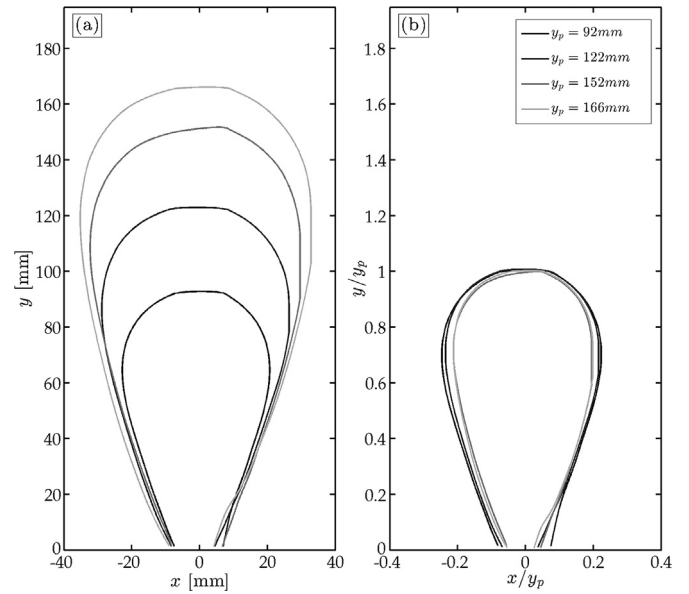
Fig. 6. Geometry of the vortex ring bubble calculated at plume heights for Ra = 1.36 \times 10^6 (a), and the same geometries normalised by the plume height (b).
