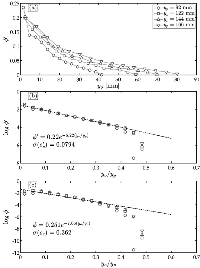
Fig. 5. Variation in the composition of the plume for four different plume heights for Ra = 1.36 \times 10^6 (a); \phi' is the normalised number of tracers which originated from a given height, y_o . The exponential distribution of tracers is clear in (b), in which the height of the tracer origin is normalised by the plume height. The three-dimensional distribution, which accounts for the radial position of tracers (Equation (12)), is shown in (c).
