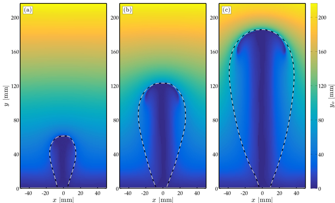
Fig. 3. Tracer fields showing the vertical origin of material at y_p = 60.8 mm (a), 122.1 mm (b), and 185.2 mm (c), for Ra = 1.36 \times 10^6 . The vortex ring bubble is shown by the back and white dashed lines, and aligns with the boundary between ambient fluid and that derived from very deep in the fluid domain.
